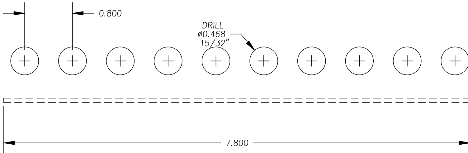
EXP-BUS 2 MOUNTING TEMPLATE 100% SCALE
