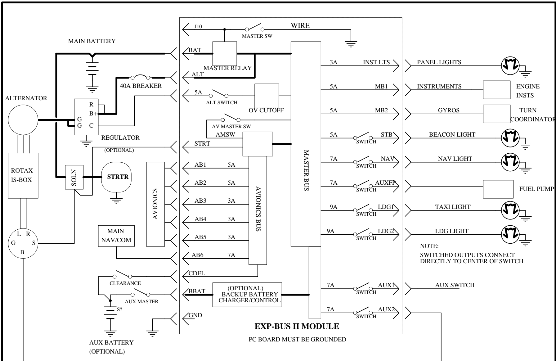
TYPICAL INSTALLATION ROTAX 912/914
